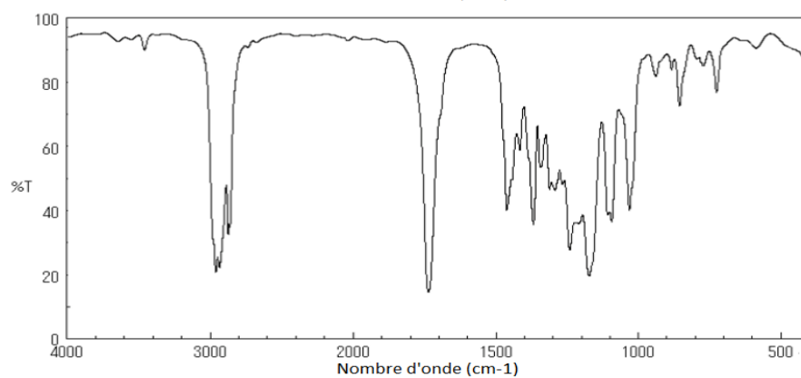
Spectre 2
