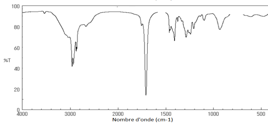
Spectre 3
