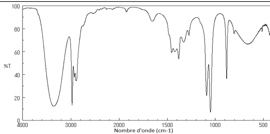
Spectre 1
