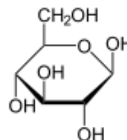
D-Glucose
